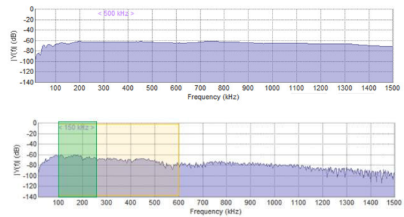
Figure 11: The calibration pulse spectrum (top) and spectrum of the real PD (bottom) measured on a stator winding.
