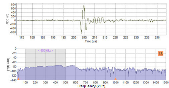
Figure 14: The real PD pulse (top) and its frequency spectrum (bottom) measured on a power transformer.
