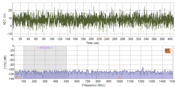
Figure 6: White noise (top) and its FFT (bottom).
