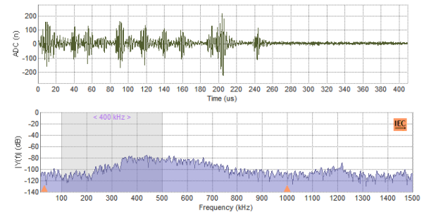
Figure 7: Switching noise (top) and its FFT (bottom).
