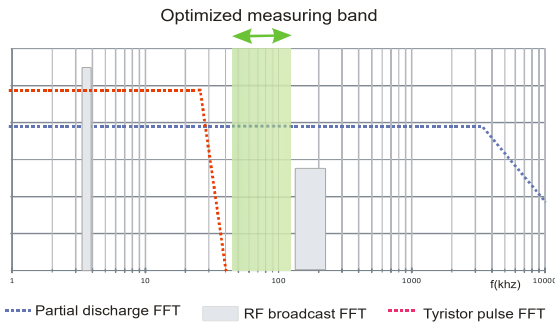
Figure 5: Typical frequency spectrum of various signal sources.
