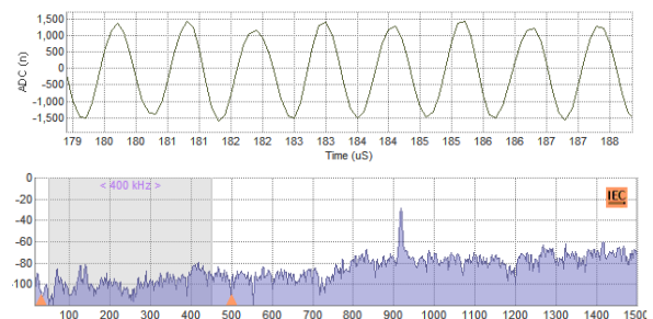
Figure 9: Sinusoidal noise (top) and its FFT (bottom).
