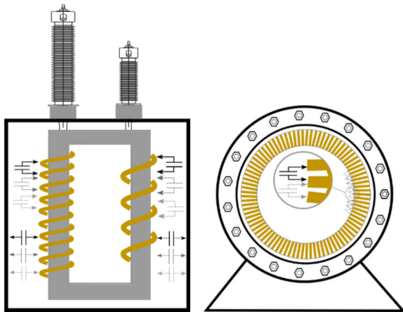
Figure 1: The stray capacitances in a transformer and a rotating machines stator winding.
