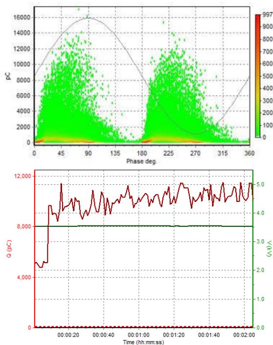
Figure 13: PRPD pattern (top) and Q(t)&U(t) diagram (bottom) measured in the frequency range 100 – 250 kHz
