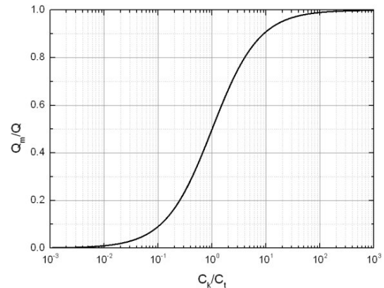
Figure 4: Sensitivity of the measurable charge in dependence of the C_k to C_t ratio.
