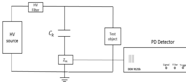
Figure 3: Schematic of the PD measurement setup.
