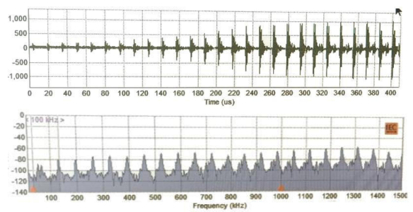
Figure 8: Switching noise from switching power supply as e.g. laptop or computer (top) and its FFT (bottom).
