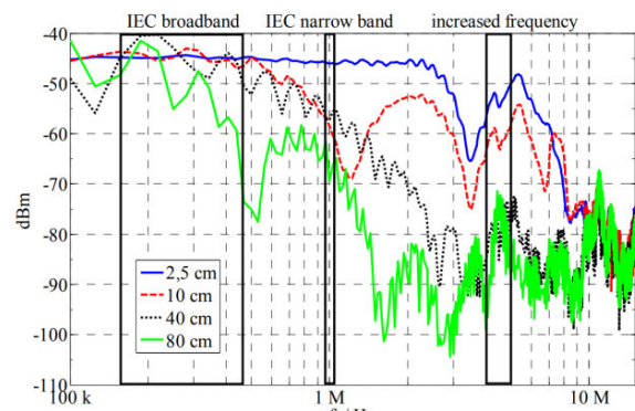
Figure 2: The pulse spectrum of a PD source simulated at different winding positions [7].
