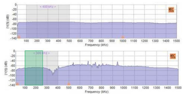
Figure 10: The frequency spectrum of an ideal calibration pulse (top) and with resonance at 350 kHz (bottom).
